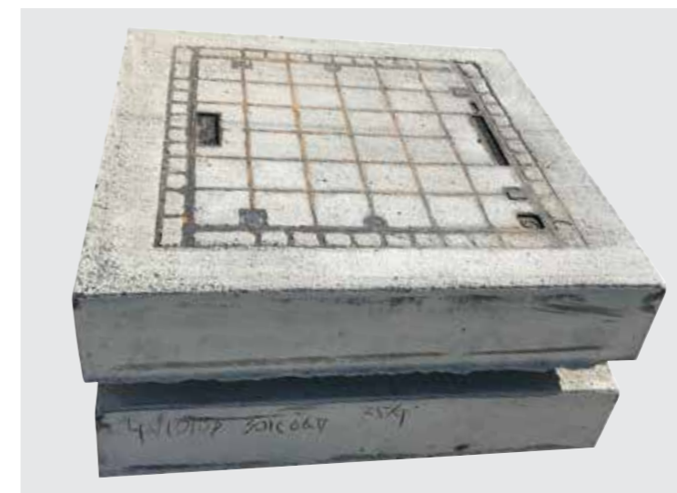
900mm x 900mm x 200mm Cast Iron Class D – 600mm x 600mm Infilled Concrete with Concrete Surround
